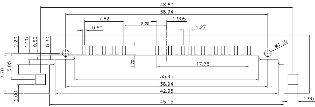
RECOMMENDED PCB LAYOUT(1t)
